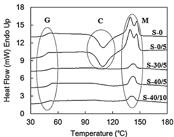
Fig. 6. The DSC heat flows of blended materials.
