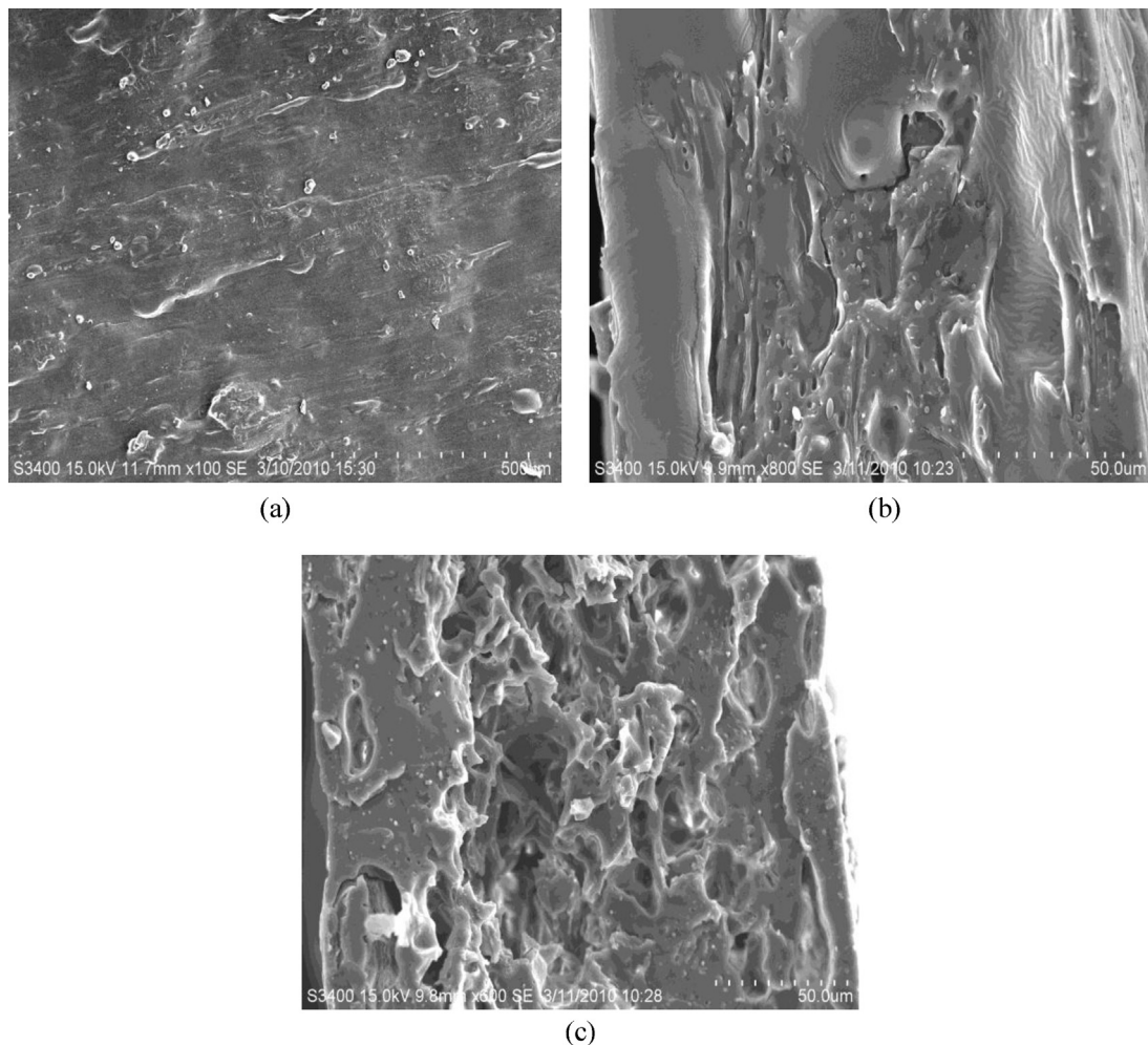
Fig. 2. The morphologies of the surface and fracture of PLA/starch/chitosan antimicrobial materials (S-40/5) before and after releasing: (a) is the surface before releasing; (b) is the fracture before releasing; and (c) is the fracture after releasing.
